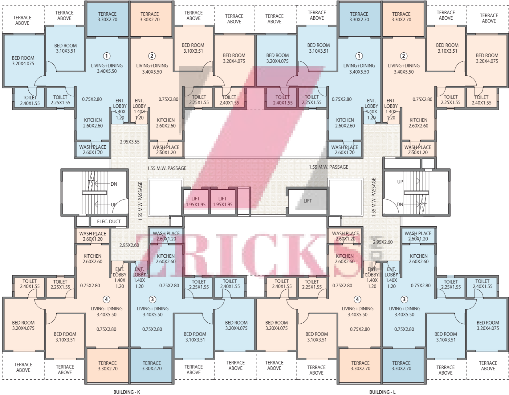
"Building K & L - 2 BHK - Typical Odd Floor Plan"
